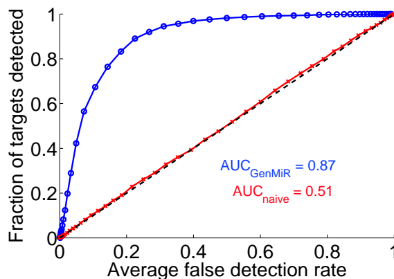
Figure 4: Fraction of candidate targets detected ( \{\# \text{ of candidate targets detected}\} / \{\# \text{ of candidate targets}\} ) VS. average false detection rate ( \{\text{Average } \# \text{ of permuted targets detected}\} / \{\# \text{ of candidate targets}\} ) using both GenMiR scoring (circle) and naive Pearson correlation scoring (cross), with areas under the curves (AUC) shown.
