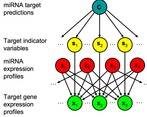
Figure 3: Bayesian network used for detecting miRNA targets: each mRNA transcript is assigned a set of indicator variables which select for miRNAs that are likely to regulate it given the data.
